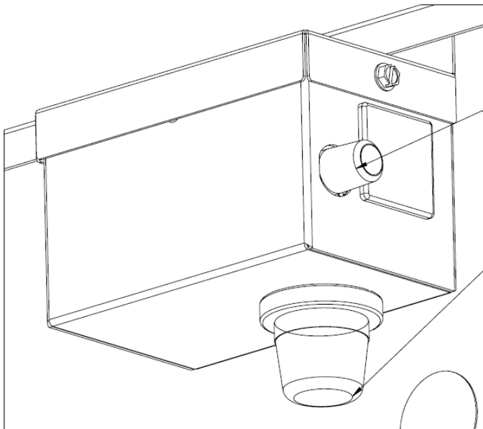
Air supply hook-up, 1/4" NPT thread.
