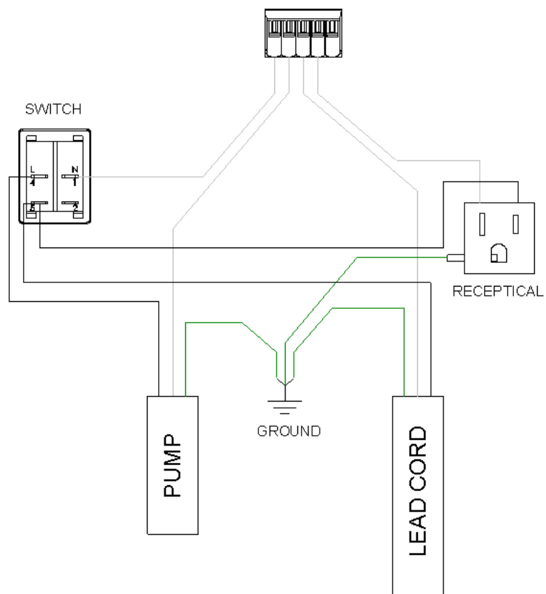
WIRE DIAGRAM
